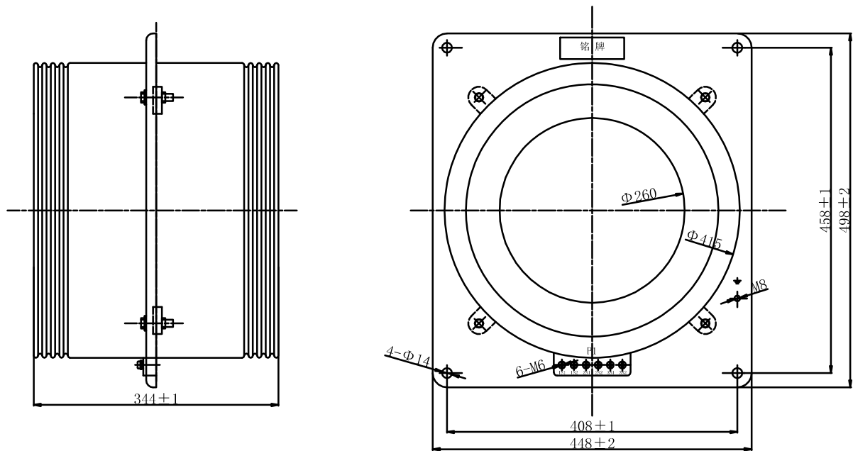
LMZBJ-10Q (Φ 260) (6000A) 净重 (Weight): 40-53kg
