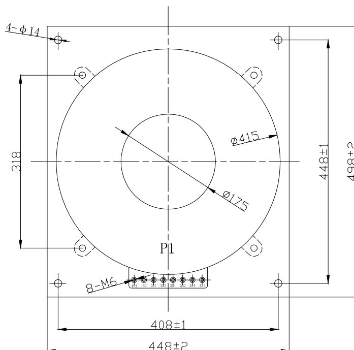
LMZBJ-10Q(8000A) 淨重 (Weight): 40-53kg
