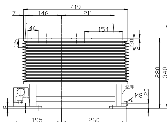
Overall dimensions
