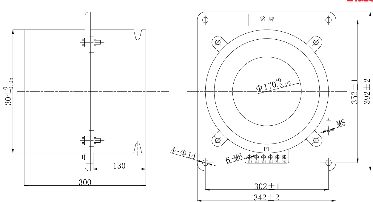
LMZBJ-10Q(4000A-6000A) 净重 (Weight): 40-53kg
